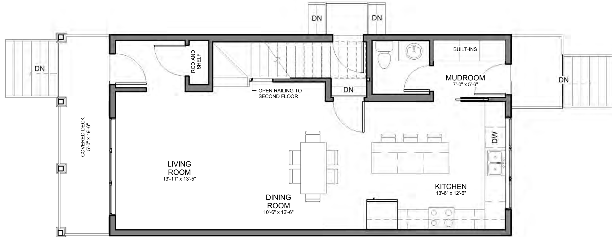
1 SALES PLAN - MAIN FLOOR 3/16" = 1'-0"
