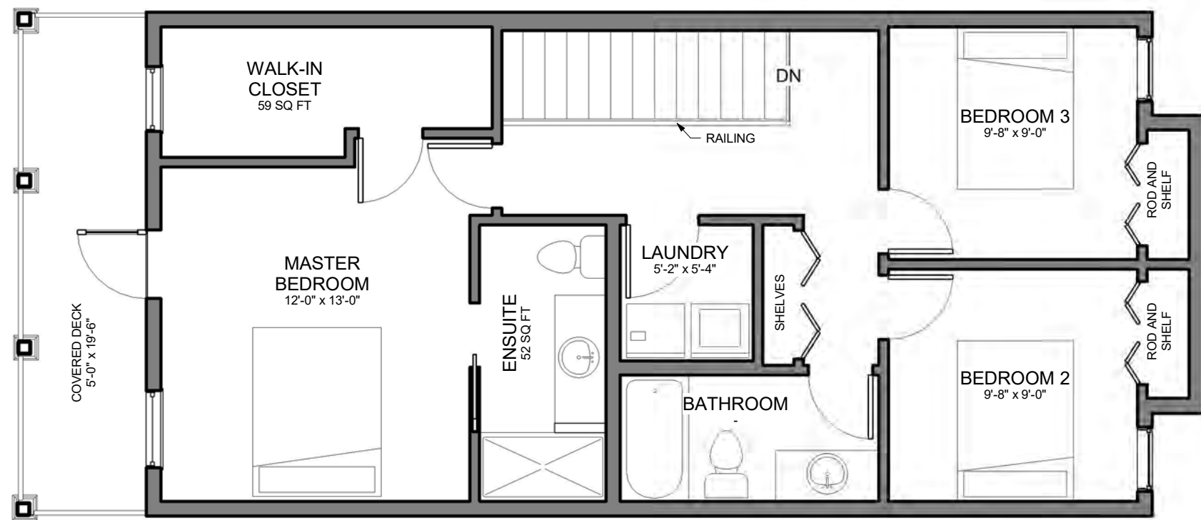
2 SALES PLAN - SECOND FLOOR 3/16" = 1'-0"
