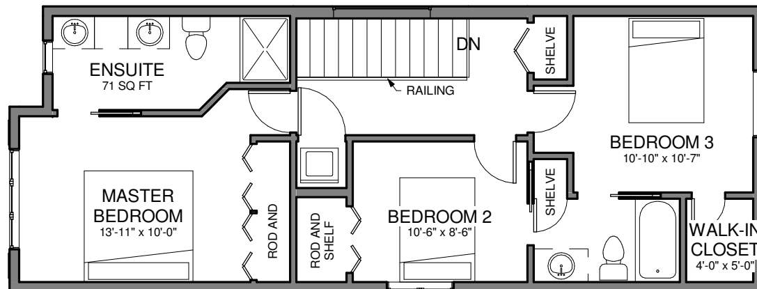
2 EVERLEE - SECOND FLOOR 1/8" = 1'-0"
