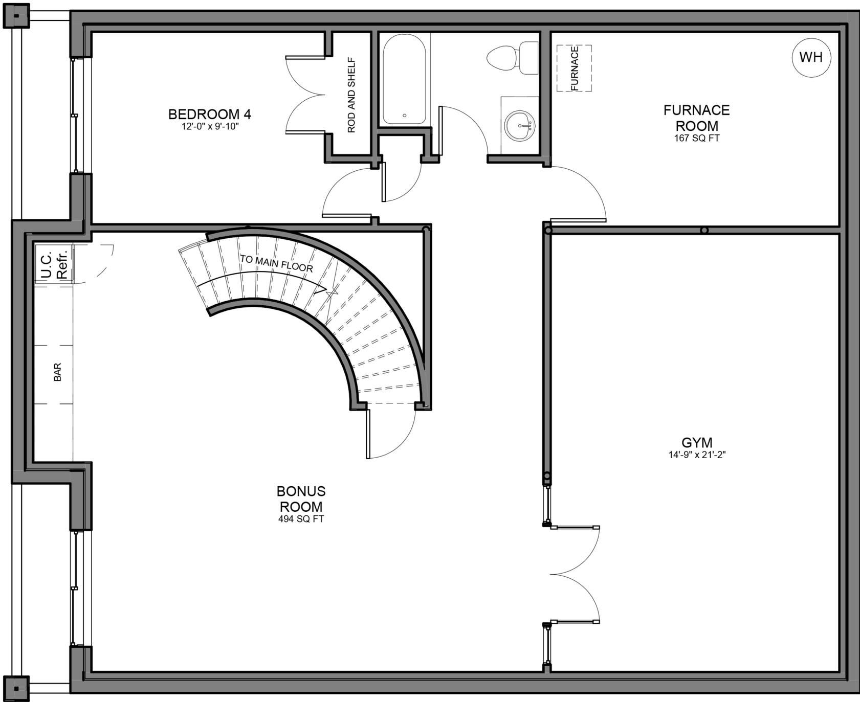
BASEMENT DEVELOPMENT PLAN
